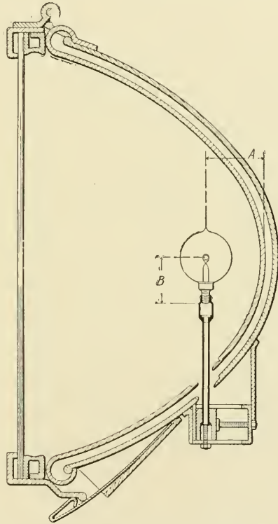
Fig. 115. Section of Incandescent Headlight
